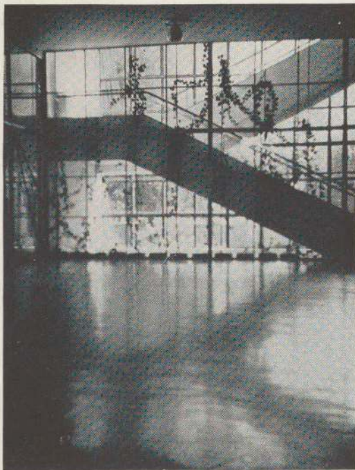
12 Library, Viipuri, 1934. Interior view of main staircase. The metal window divisions form a trellis for the vines which are planted in boxes along the landings.
